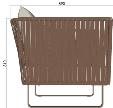
SIDE / LATERAL
